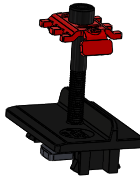
Shared Rail Mid Clamp
