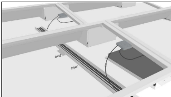
Examples of wire installation in RayTray underneath modules.
