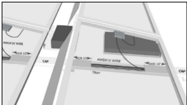
Examples of wire installation in RayTray underneath modules.
