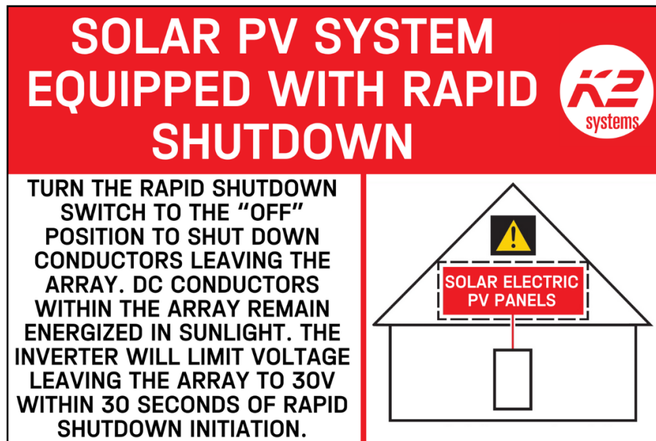
Rapid Shutdown Switch Label, no MLPEs used.
