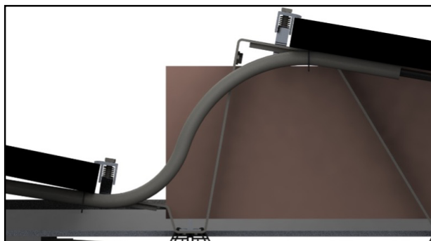
Examples of row-to-row wire installation through listed conduit.
