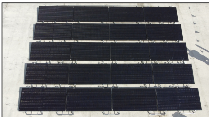
All wiring managed under module; required conduit, raceways, and cable ties are not shown in the example above.
